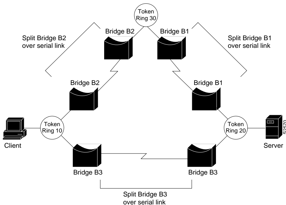
Figure 3-7 Redundancy in a Pure SRB Network
