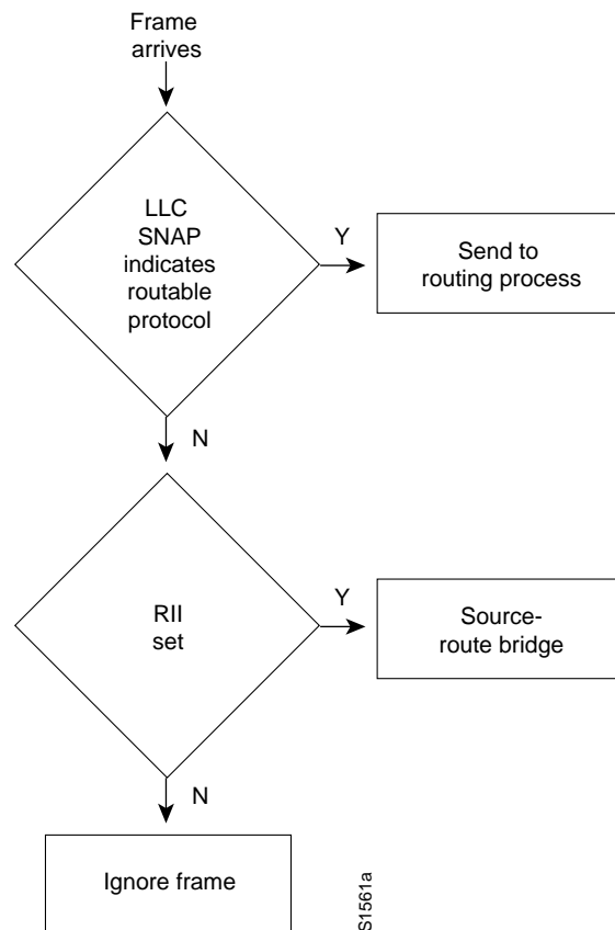
Figure 3-16 Process for Identifying Routable Versus SRB Packets
