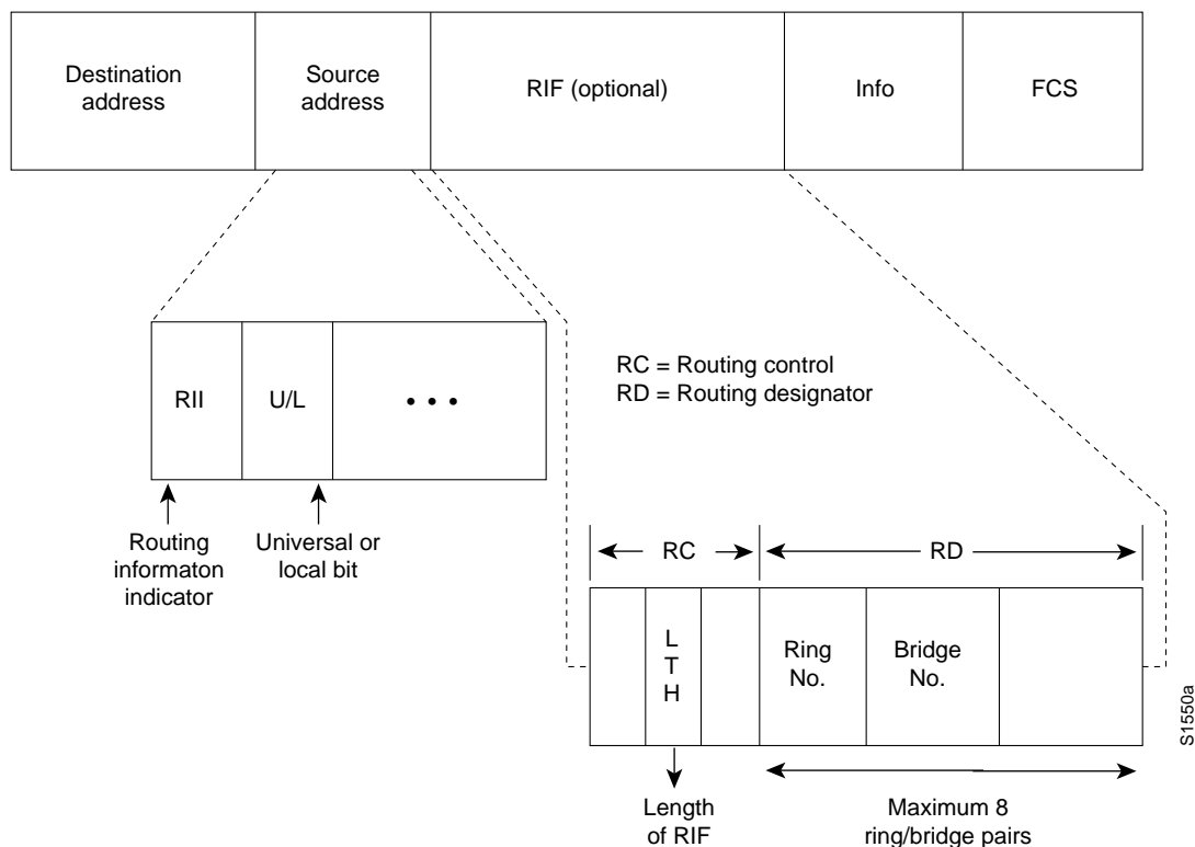
Figure 3-17 RIF Format
