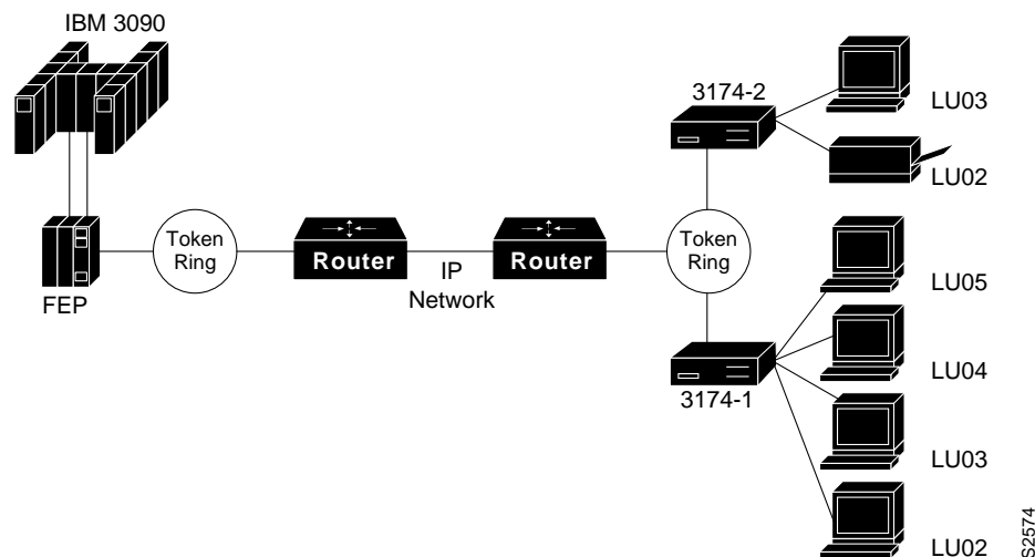
Figure 3-36 LU Prioritization for RSRB
