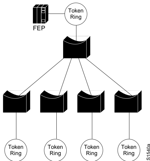
Figure 3-31 Hierarchical Topology Featuring a Single FEP
