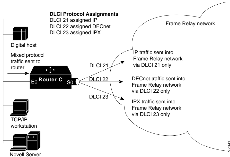
Figure 6-12 Virtual Interfaces Assigned Specific Protocols
