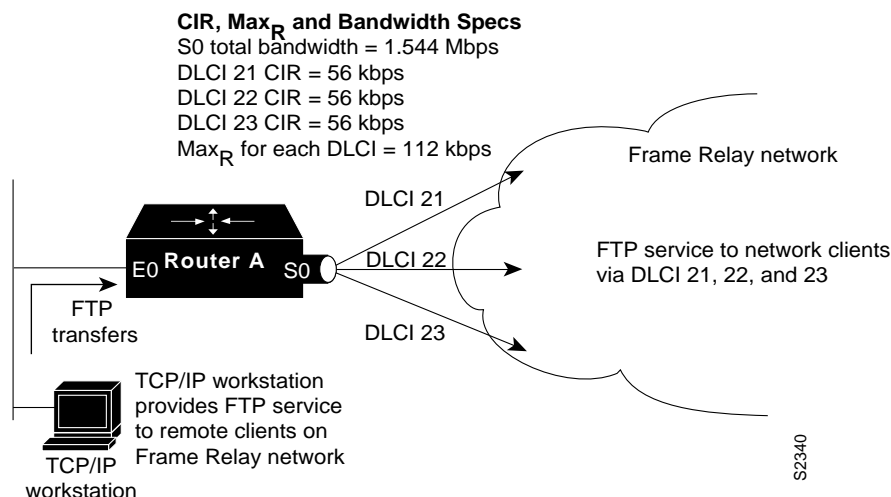
Figure 6-11 Example of a CIR and CBR Traffic Limiting Situation
