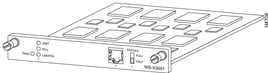
Figure 5-20 100Base-TX Module
