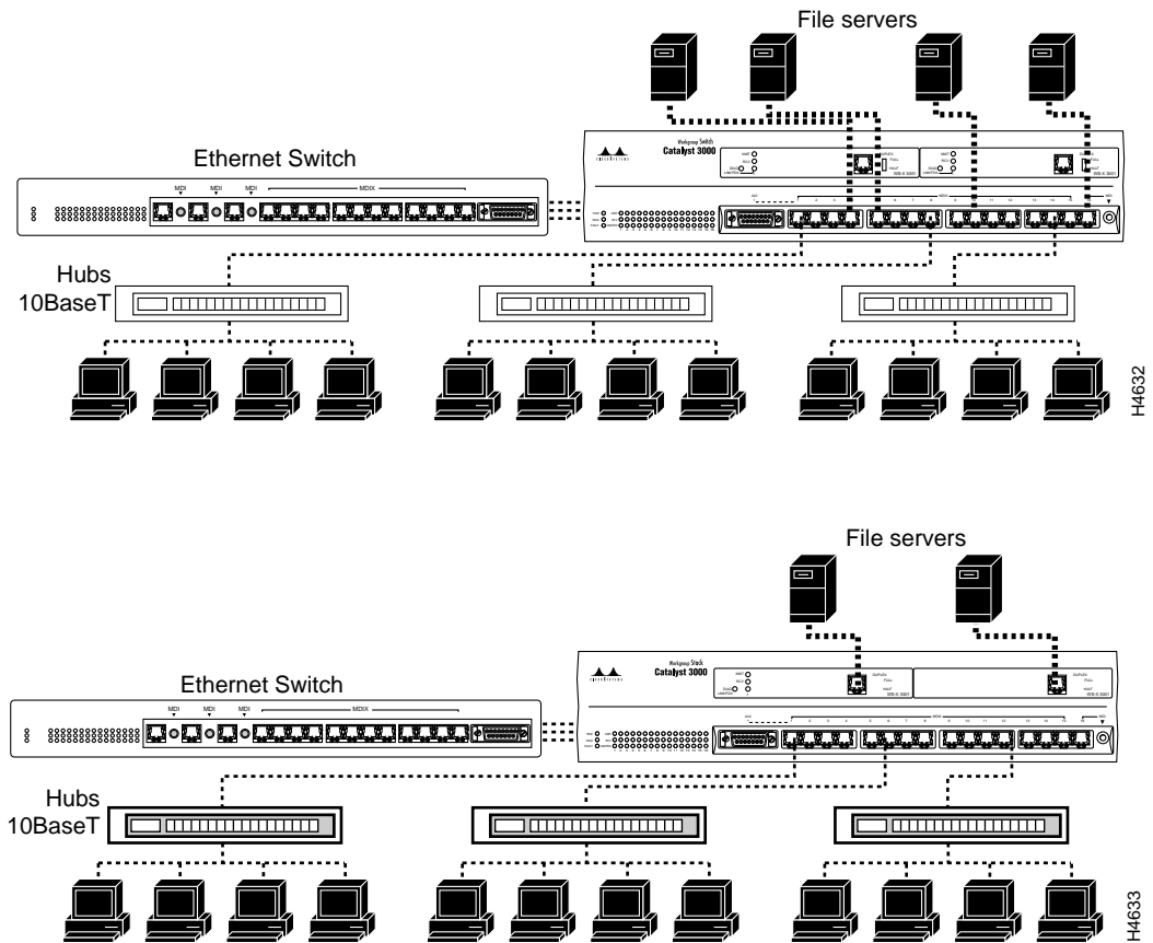
Figure 5-10 Examples Of Different Network Connections
