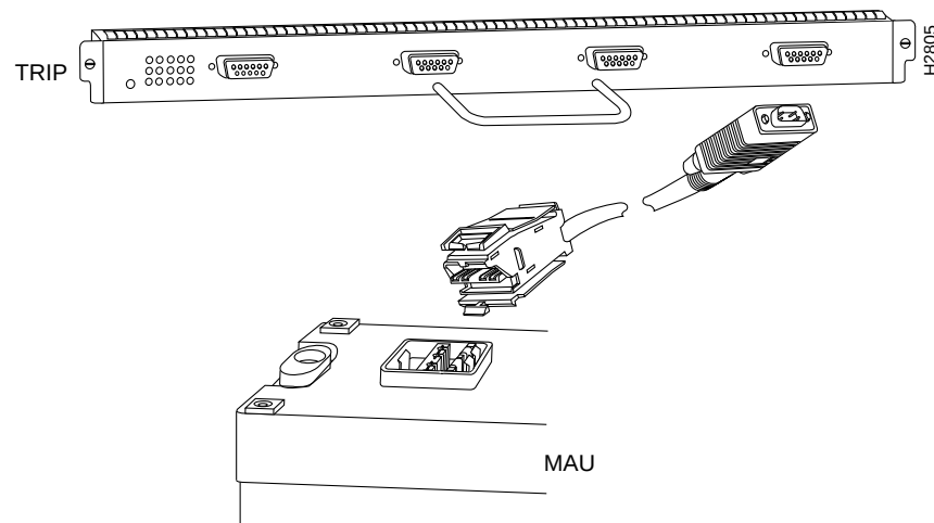
Figure 4-2 Connecting Cables to the TRIP
