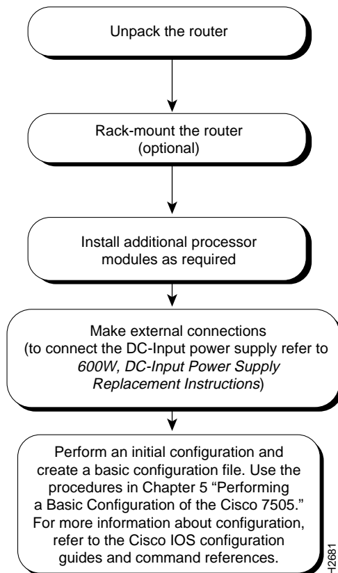
Figure 2-1 Installation Flowchart
