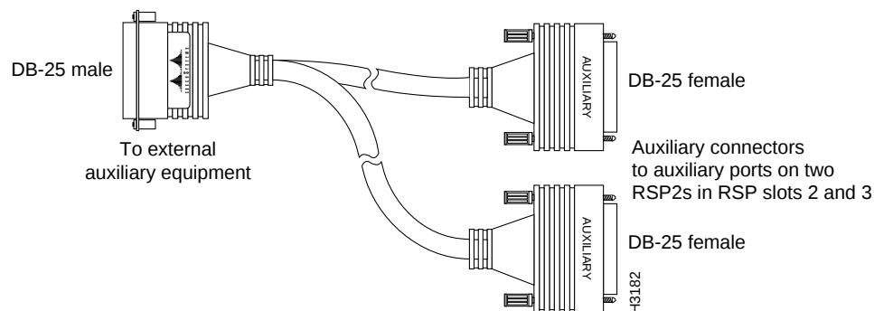
Figure 4-22 Auxiliary Y Cable (CAB-RSP2AUX=)
