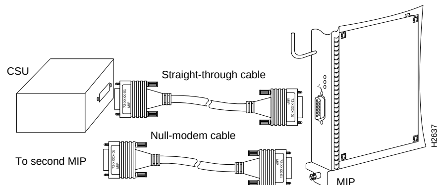
Figure 4-19 Connecting Cables to the MIP
