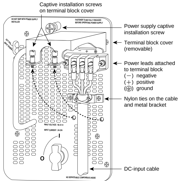
Figure 4-23 Installing the Power Cable Leads, Nylon Ties, and Cover
