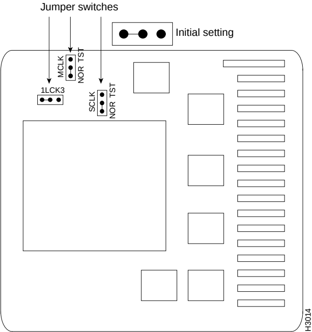
Figure 3-6 Motherboard Jumper Switches
