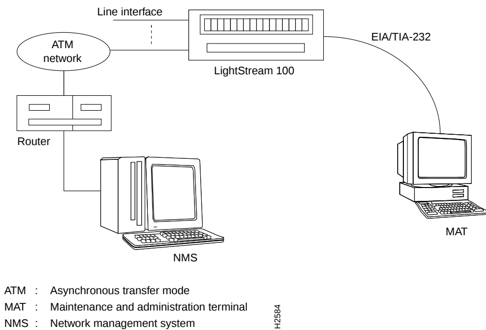
Figure 3-15 LightStream 100 ATM Switch to Console Terminal and NMS Connection
