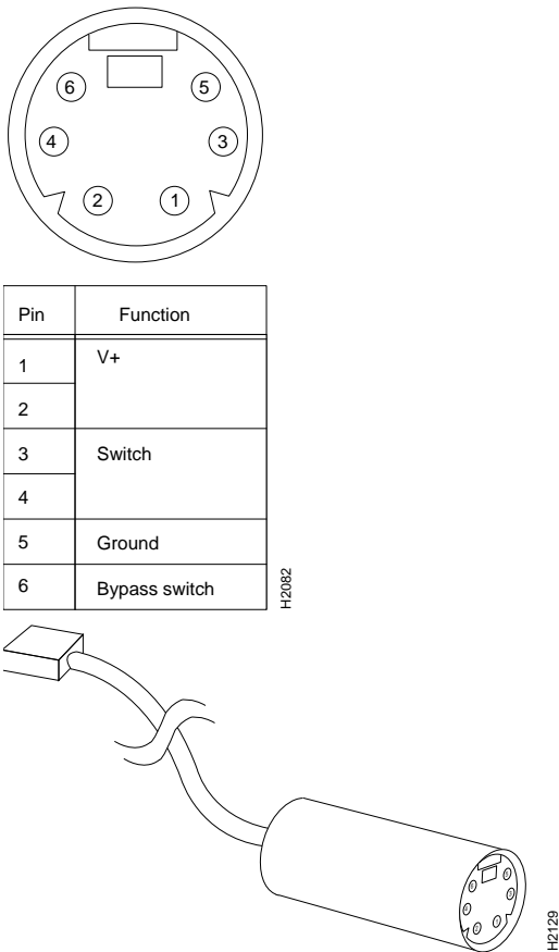
Figure D-1 Bypass Connector Pinouts
