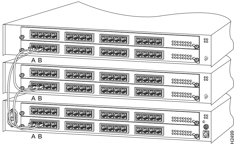
Figure 4-2 Concentrators in a Dual-Ring Configuration—CDDI Shown
