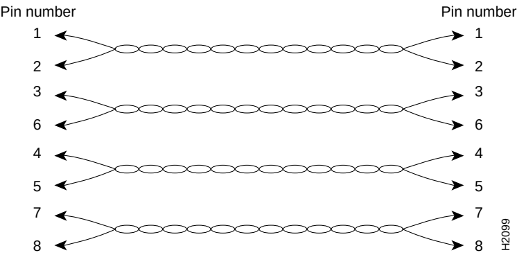
Figure A-2 10BaseT Twisted-Pair Wiring Configuration— Straight-Through Cables
