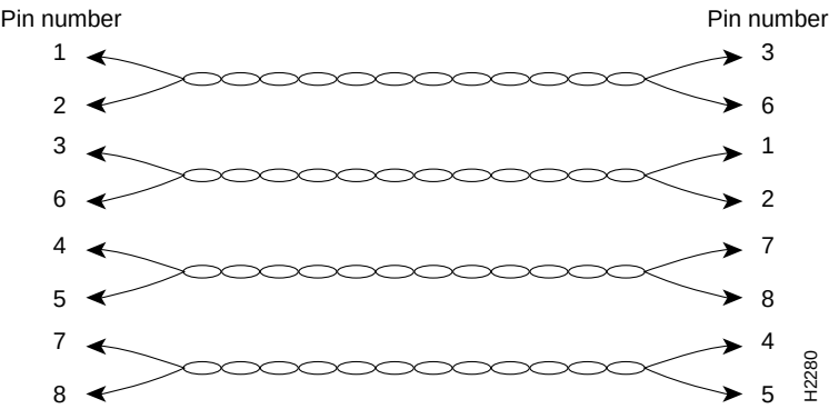
Figure A-3 10BaseT Twisted-Pair Wiring Configuration— Cross-Connect Cables
