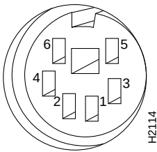
Figure A-4 Optical Bypass Connector
