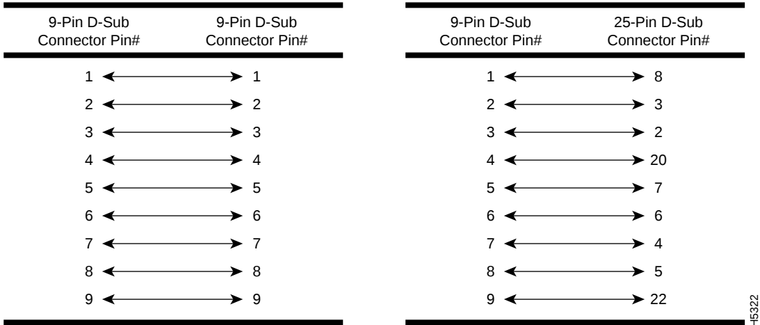
Figure A-3 Standard Modem Cable Schematic with 9- and 25-Pin Devices
