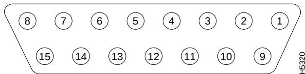
Figure A-1 AUI Connector
