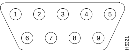
Figure A-2 Serial Connector
