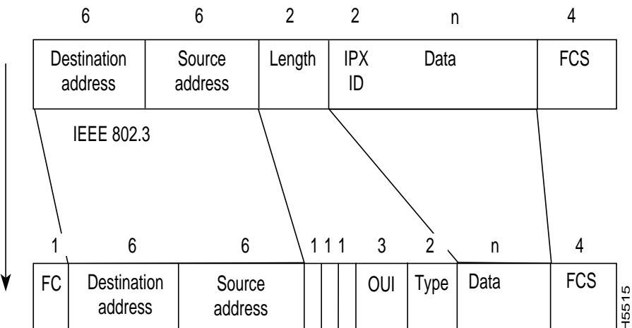
Figure C-5 Ethernet 802.3 (Novell) to FDDI-SNAP
