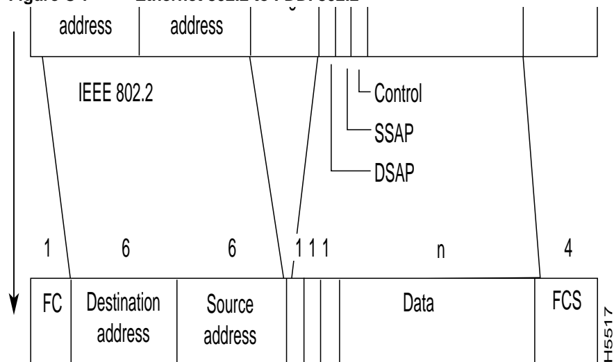
Figure C-7 Ethernet 802.2 to FDDI 802.2
