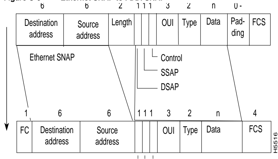
Figure C-6 Ethernet SNAP to FDDI SNAP
