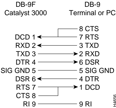
Figure A-4 RS-232-C Null Modem Cable (for Terminal/PC with 9-pin Connector)
