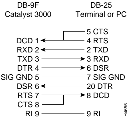
Figure A-3 RS-232-C Null Modem Cable (for Terminal/PC with 25-pin Connector)
