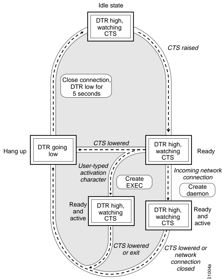
Figure 3-2 EXEC and Daemon Creation on a Line Configured for Continuous CTS
