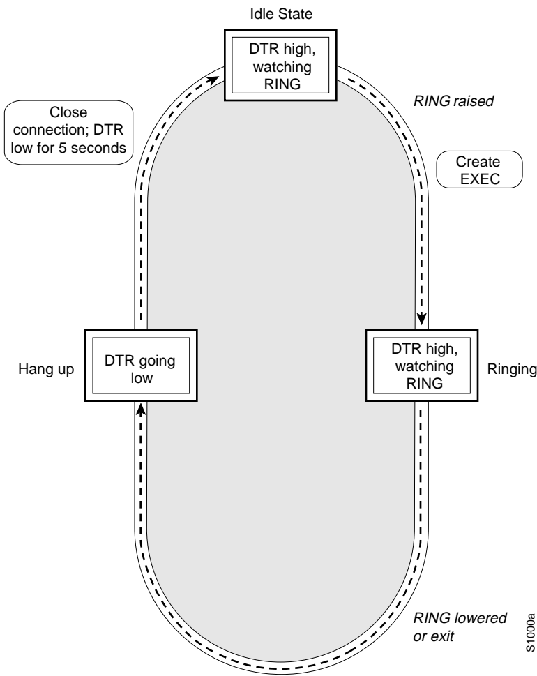
Figure 3-3 EXEC Creation on a Line Configured for a High-Speed Dial-up Modem
