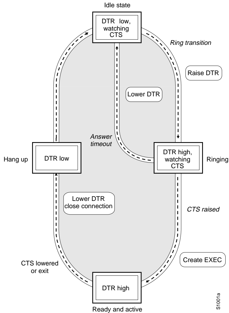
Figure 3-4 EXEC Creation on a Line Configured for Modem Callin
