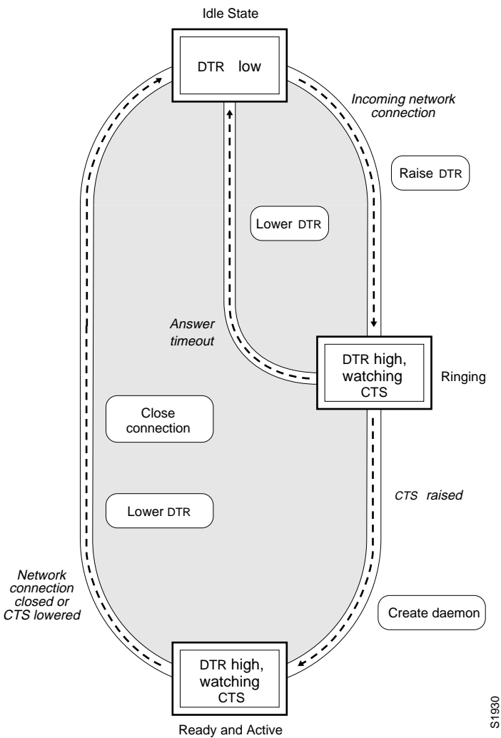
Figure 3-5 Daemon Creation on a Line Configured for Modem Callout
