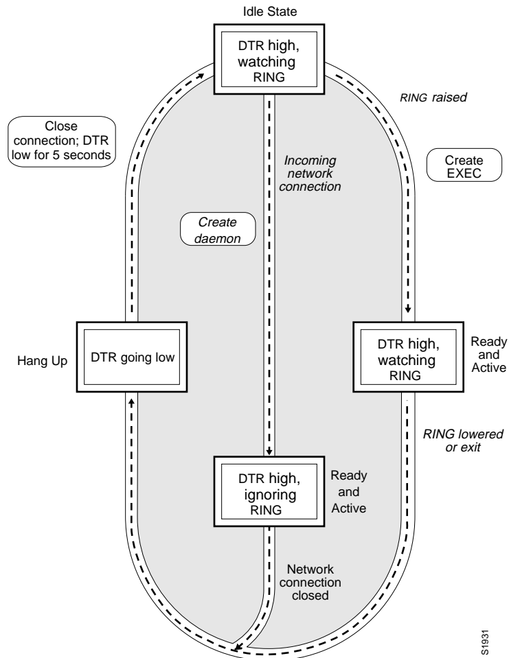
Figure 3-6 EXEC and Daemon Creation on a Line Configured for Incoming and Outgoing Calls
