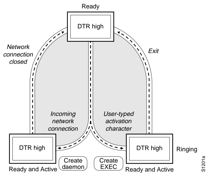
Figure 3-1 EXEC and Daemon Creation on a Line with No Modem Control
