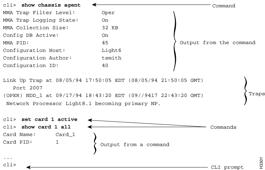
Figure 2-1 Sample Session of the CLI
