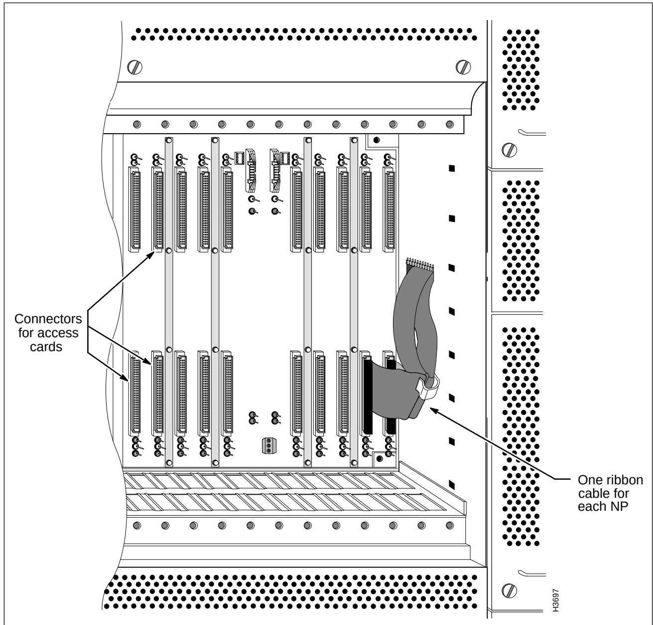
Figure 5-3 Ribbon Cables Connecting NPs to Disk Assemblies
