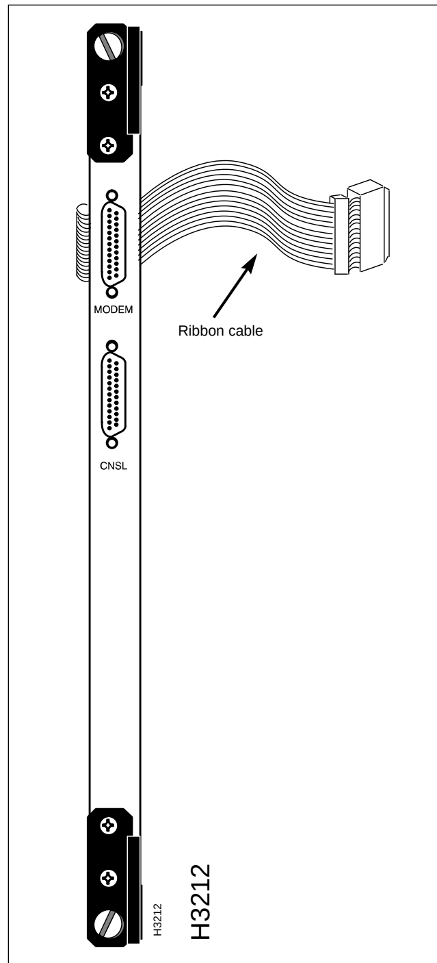
Figure 5-2 LS2020 Console/Modem Assembly
