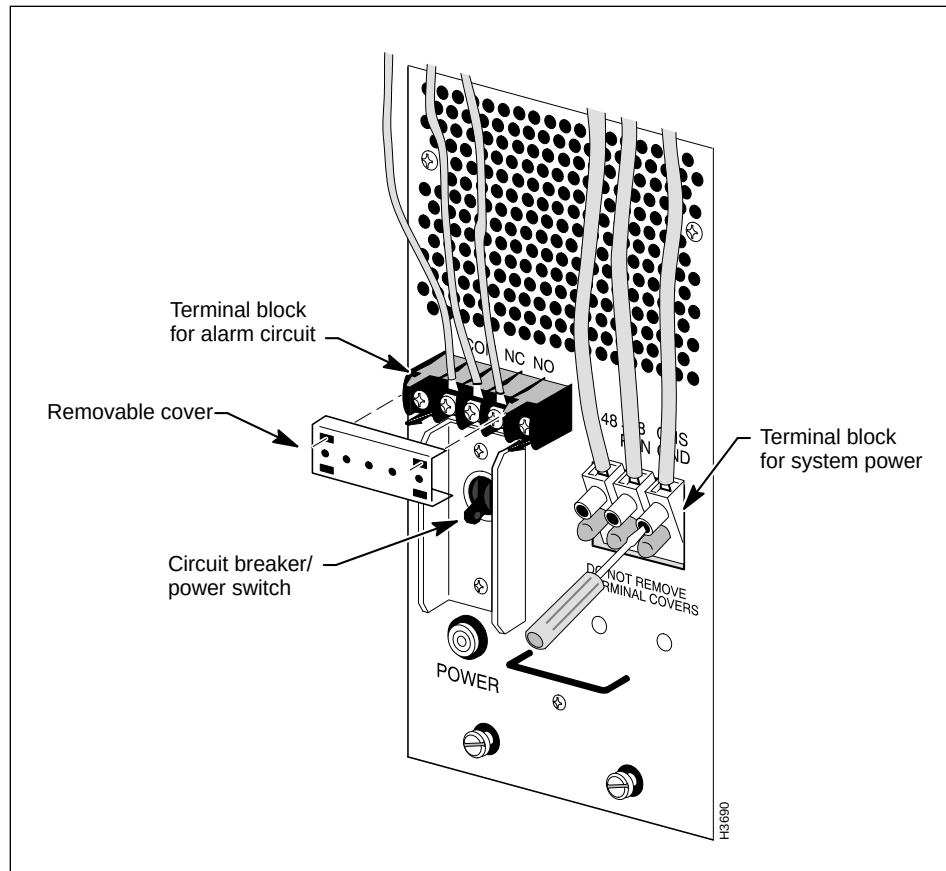
Figure 2-3 Connections to DC-powered Chassis
