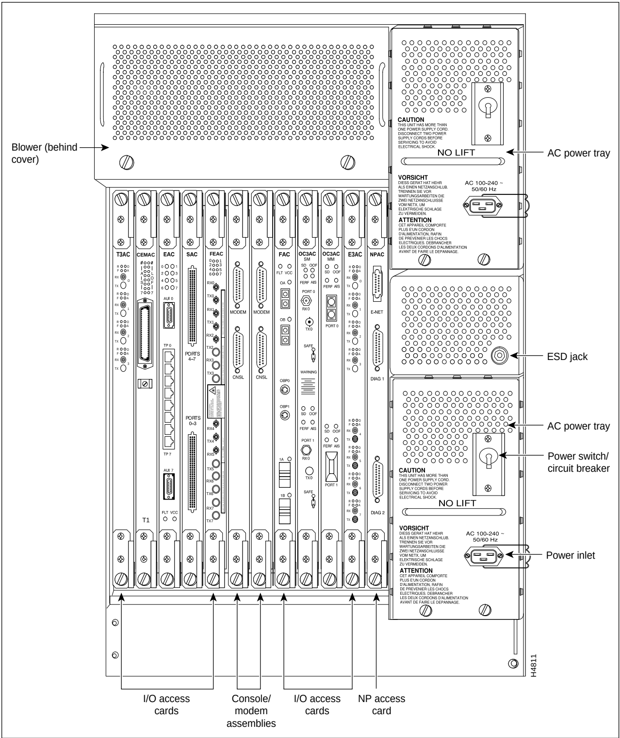
Figure 2-2 Rear View of AC-powered LightStream 2020 Chassis
