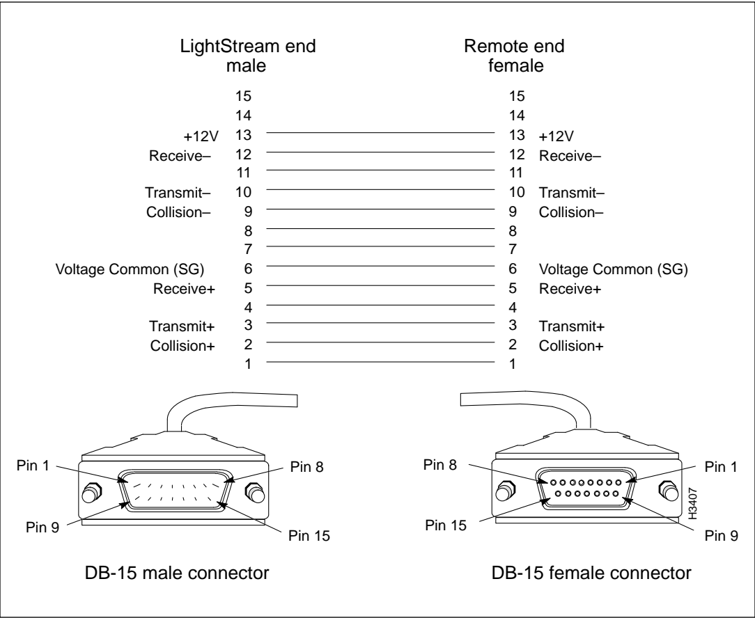
Figure 3-32 Ethernet AUI Data Cable Pin Assignments
