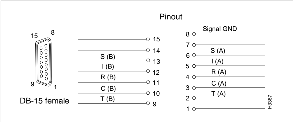
Figure 3-4 X.21 Interface Connector Pin Assignments
