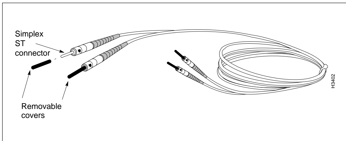
Figure 3-34 Multimode FEAC Data Cable with ST Connectors
