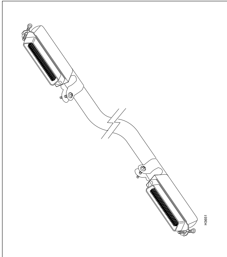
Figure 3-22 E1 Fantail Data Cable
