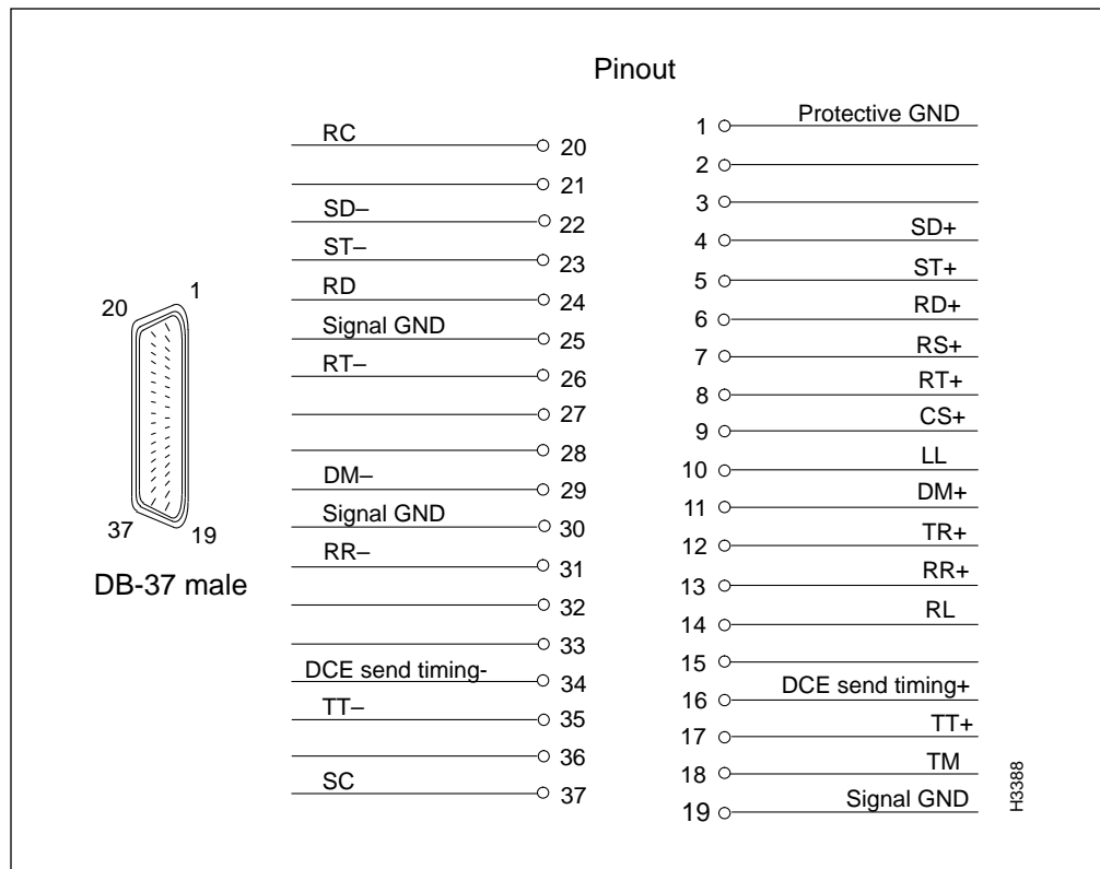
Figure 3-6 RS-449 Interface Connector Pin Assignments
