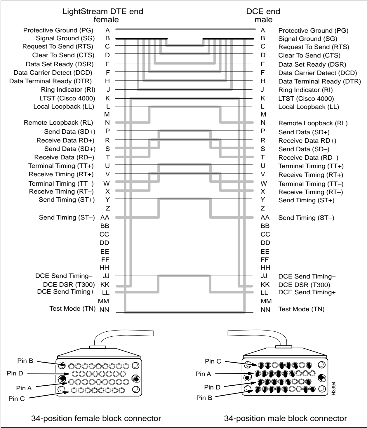
Figure 3-13 V.35 Straight-through Cable Signal Diagram
