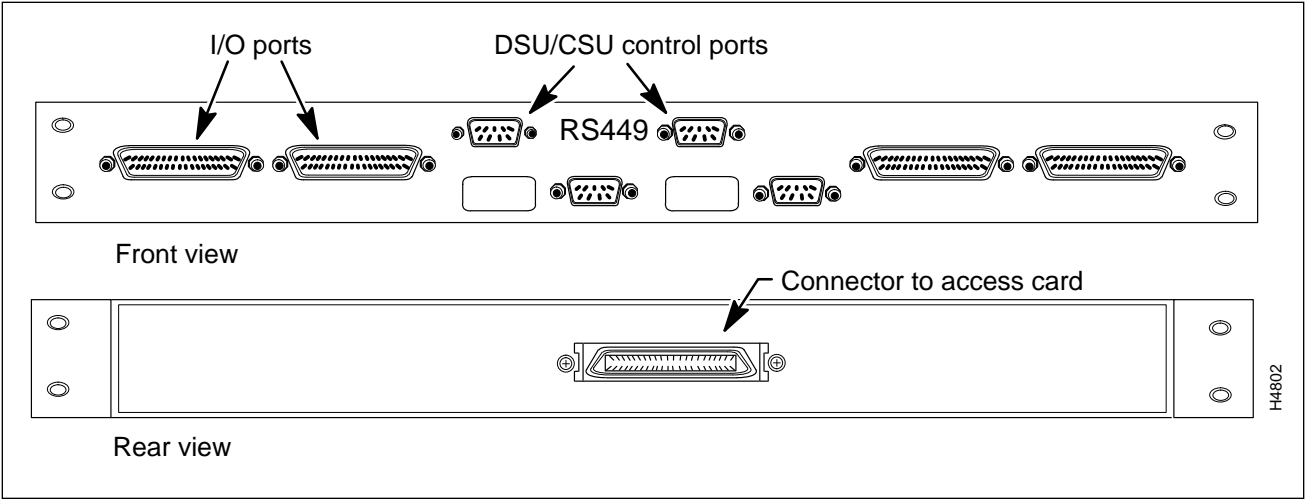
Figure 3-5 RS-449 Fantail
