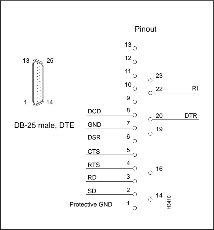
Figure 3-35 RS-232 Modem Port Pin Assignments
