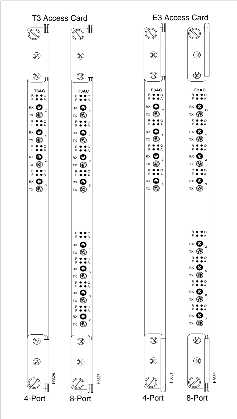
Figure 3-17 Medium Speed T3/E3 Access Cards (4-Port/8-Port)
