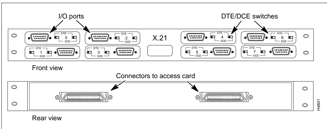
Figure 3-3 X.21 Fantail
