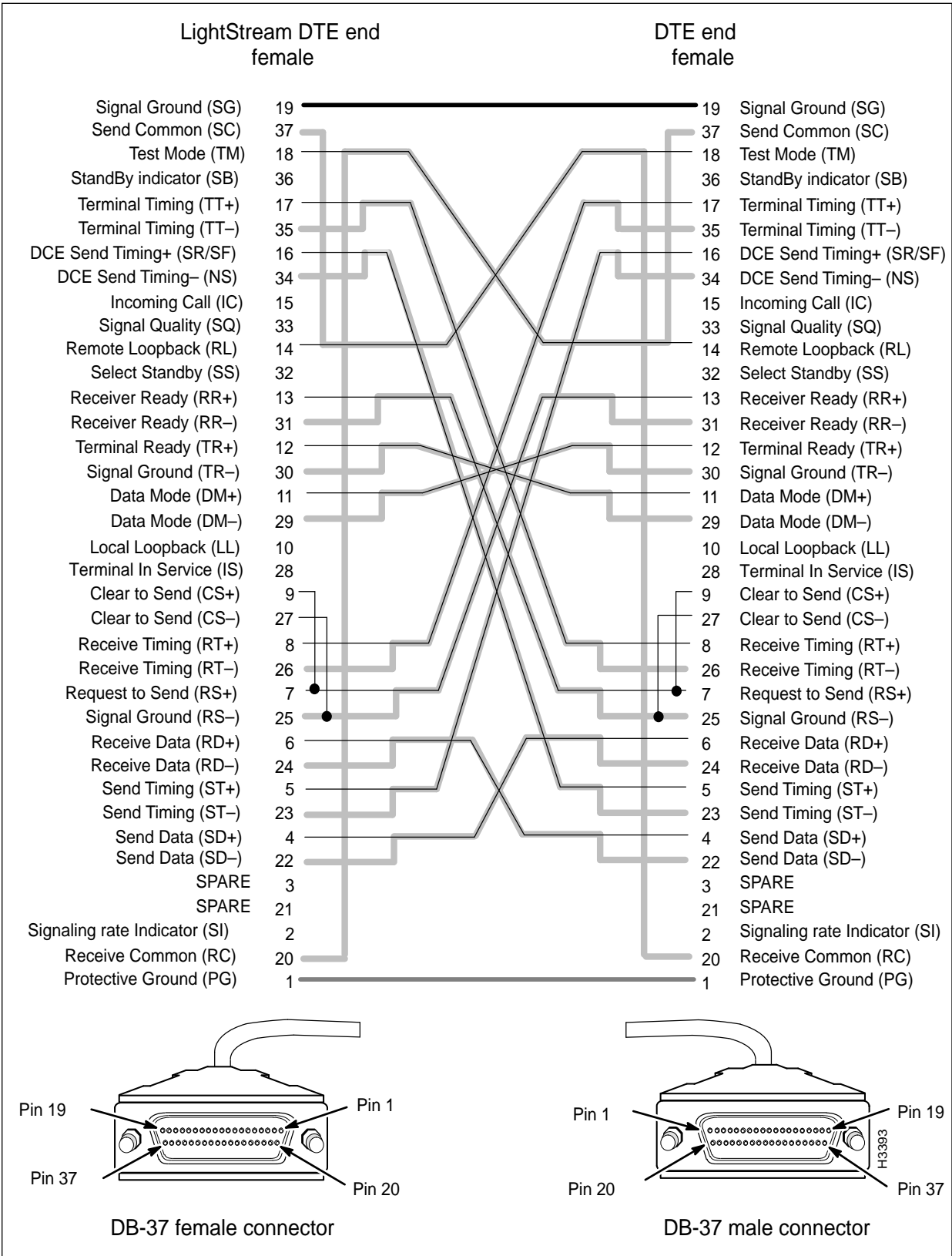
Figure 3-12 RS-449 Crossover Cable Signal Diagram
