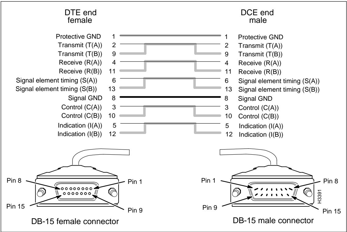
Figure 3-10 X.21 Cable Signal Diagram
