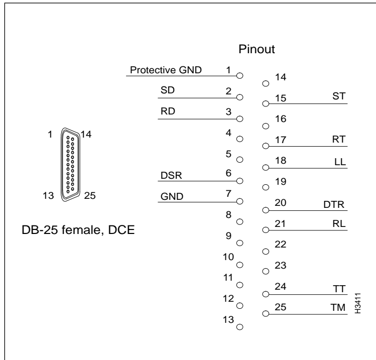
Figure 3-36 RS-232 Console Port Pin Assignments
