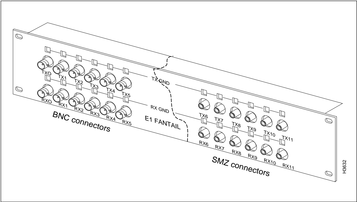
Figure 3-21 E1 Fantail
