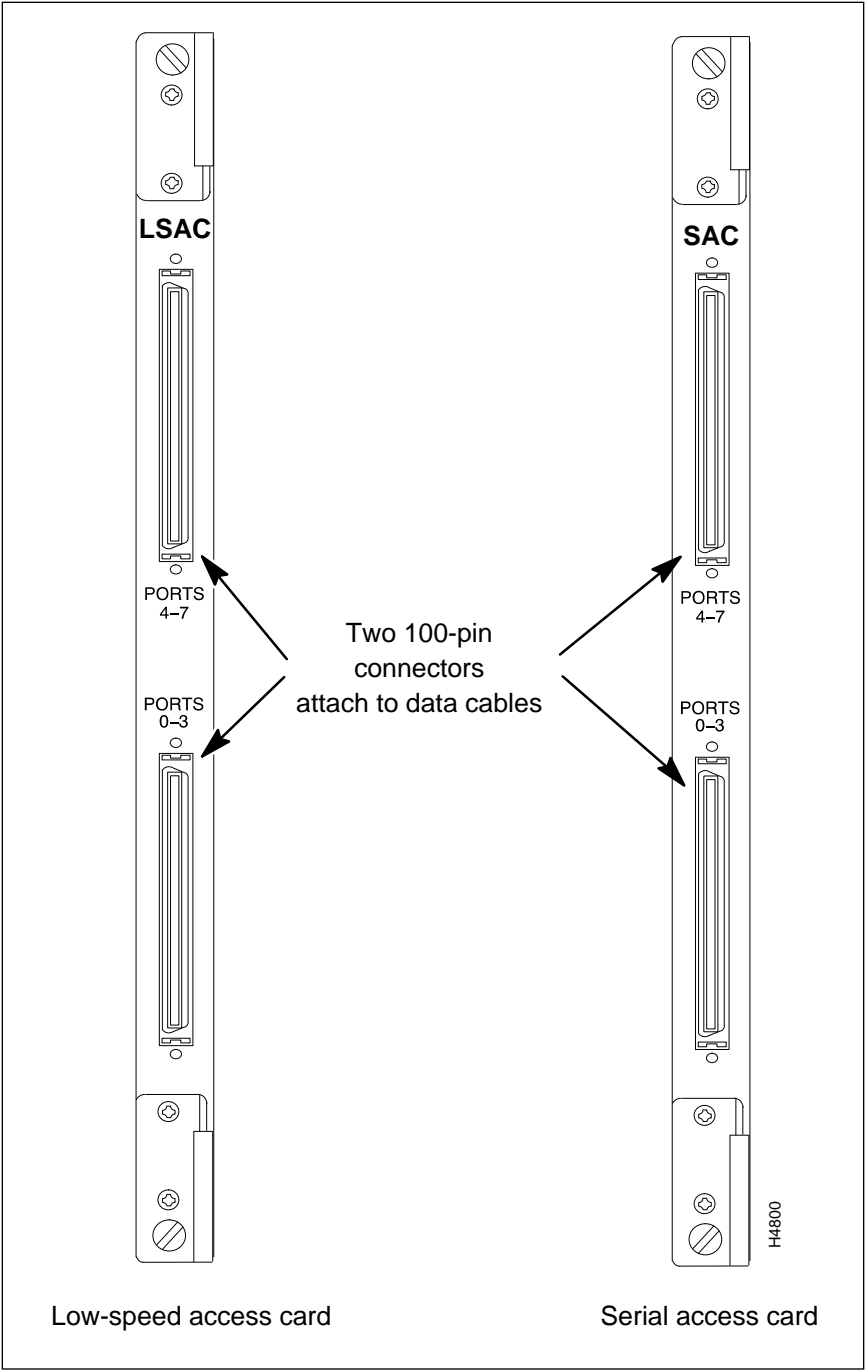
Figure 3-2 Low-Speed Access Cards
