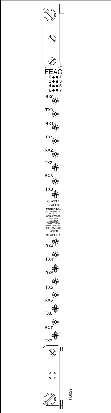
Figure 3-33 Fiber Ethernet Access Card
