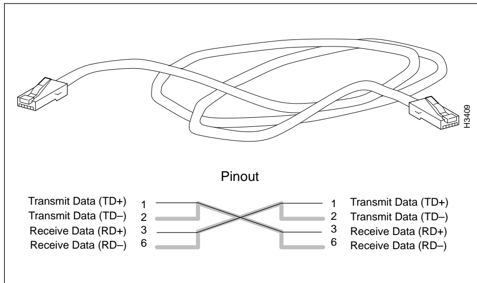
Figure 3-30 Ethernet 10BaseT Crossover Cable and Pin Assignments
