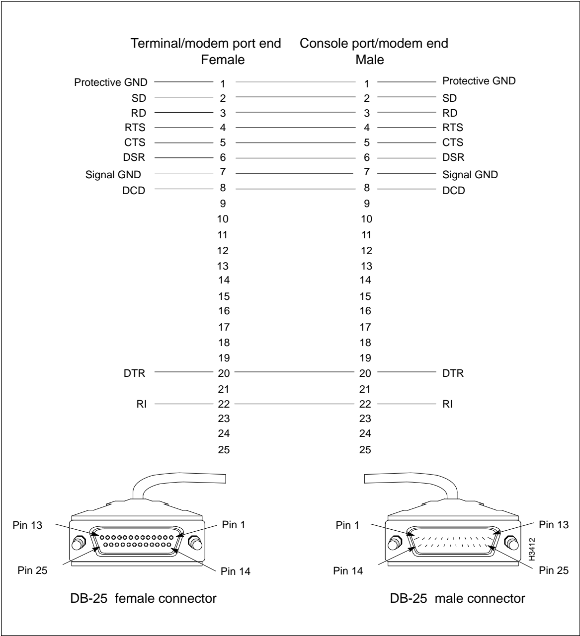
Figure 3-37 RS-232 Straight-through Data Cable and Pin Assignments
