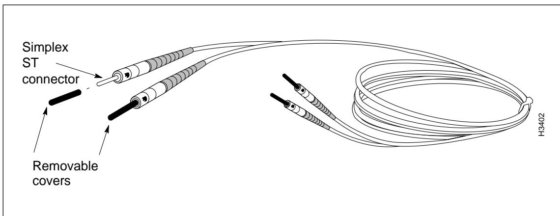
Figure 3-25 Single Mode OC-3c Data Cable with ST Connectors
