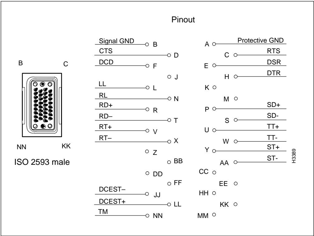
Figure 3-8 V.35 Interface Connector Pin Assignments
