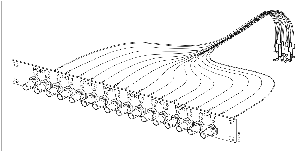
Figure 3-18 T3/E3 Fantail and Cable Harness
