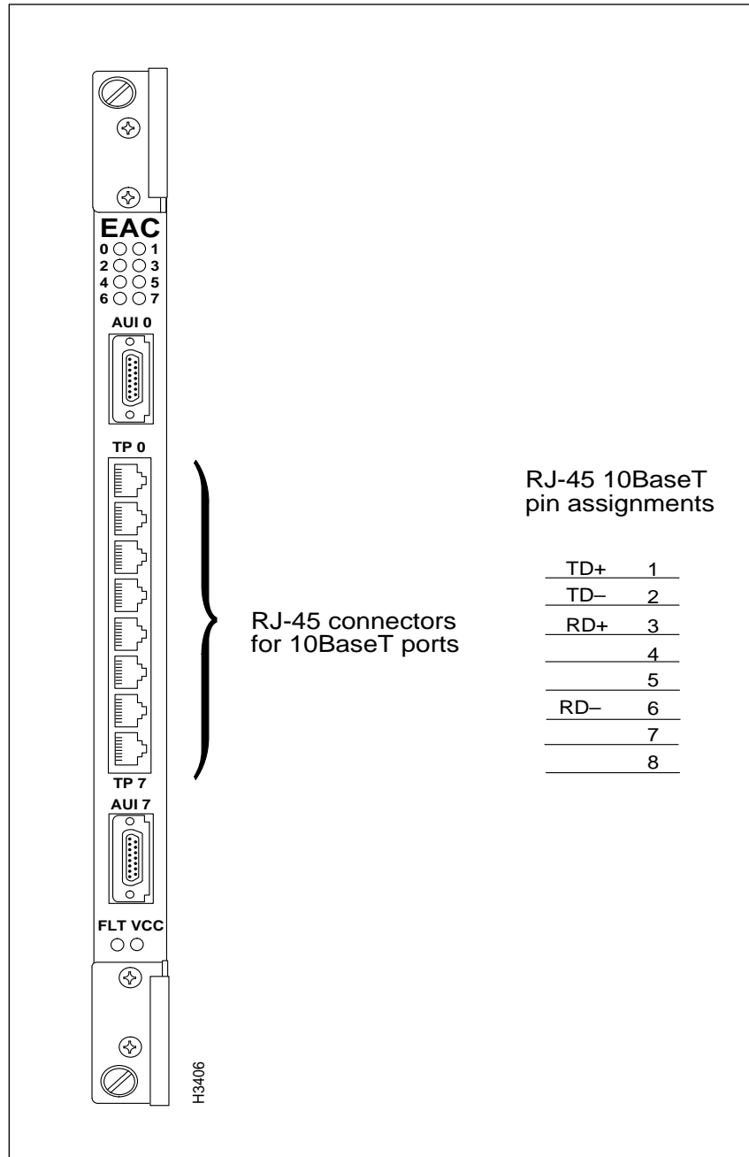
Figure 3-28 Ethernet Access Card
