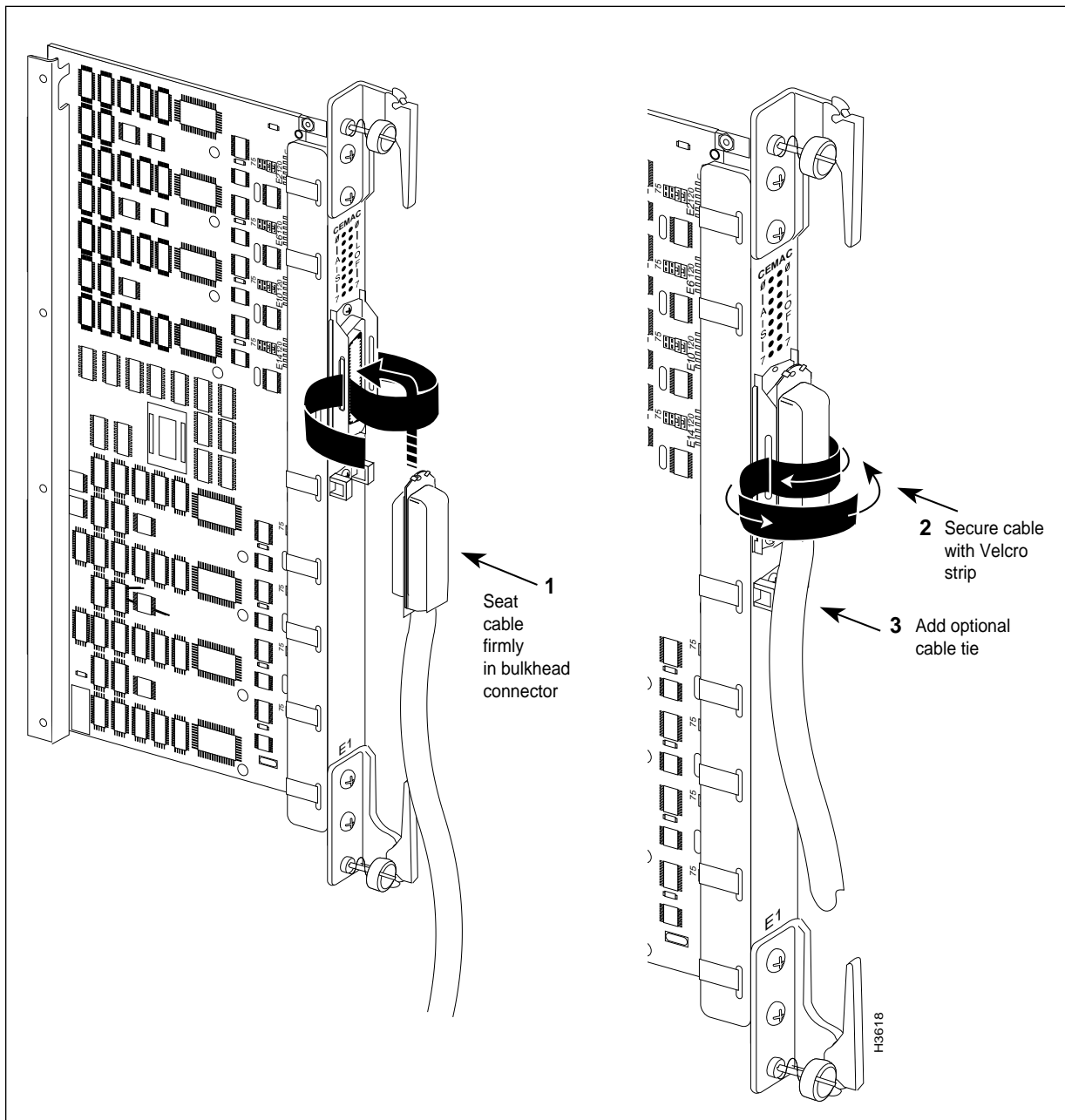
Figure 3-20 Securing Data Cable to CEMAC Bulkhead Connector
