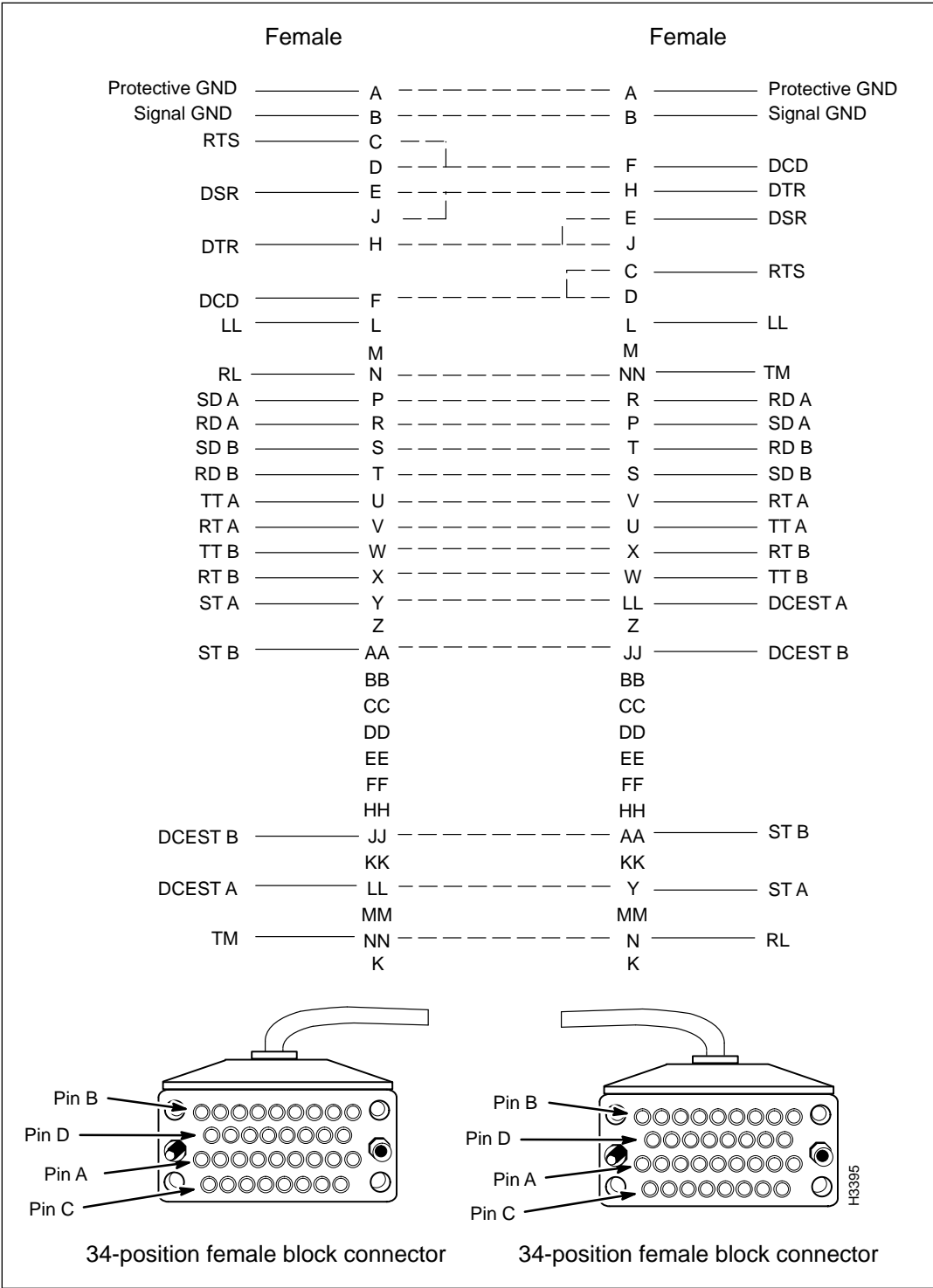
Figure 3-14 V.35 Crossover Cable Signal Diagram
