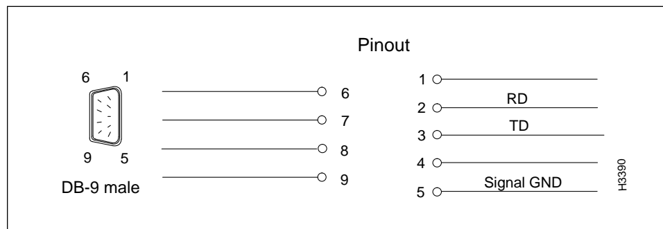
Figure 3-9 RS-232 DSU/CSU Control Port Pin Assignments
