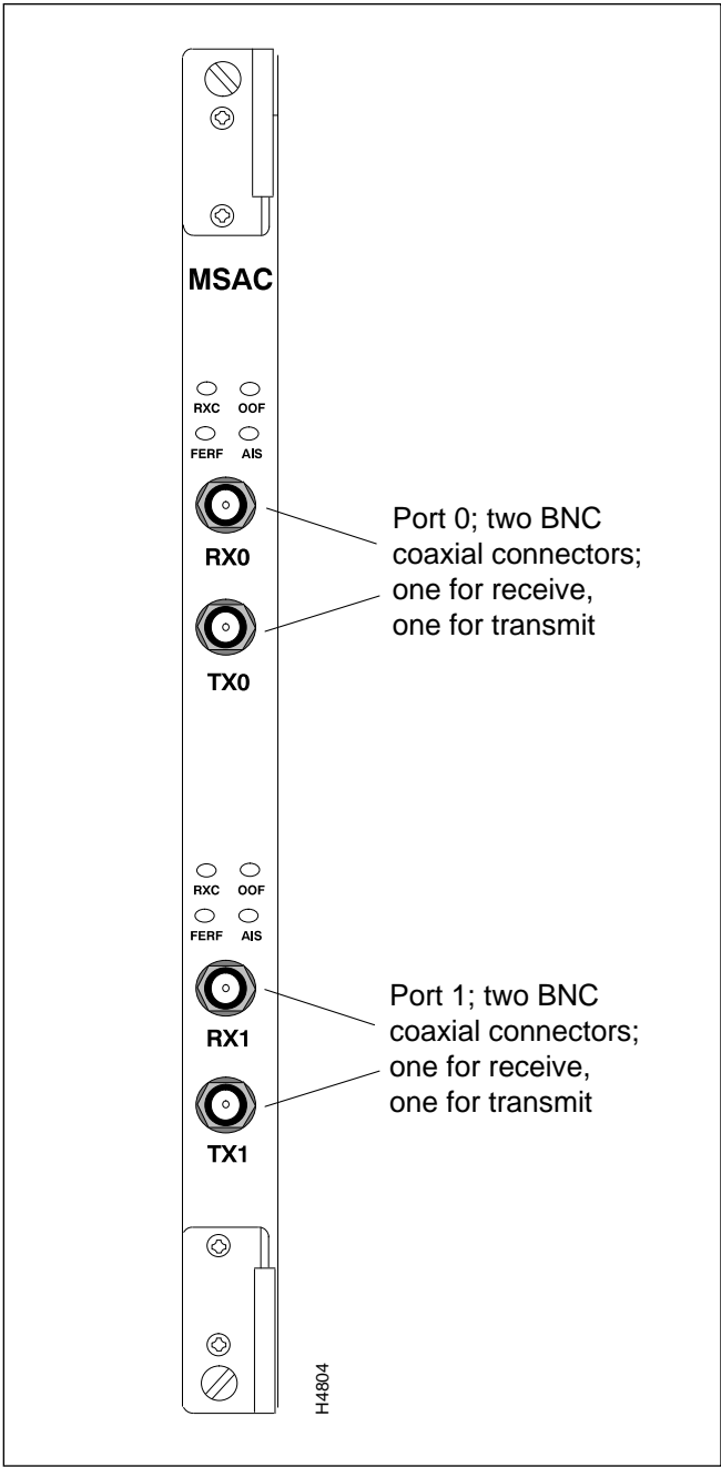
Figure 3-15 Medium-speed Access Card (2-Port)
