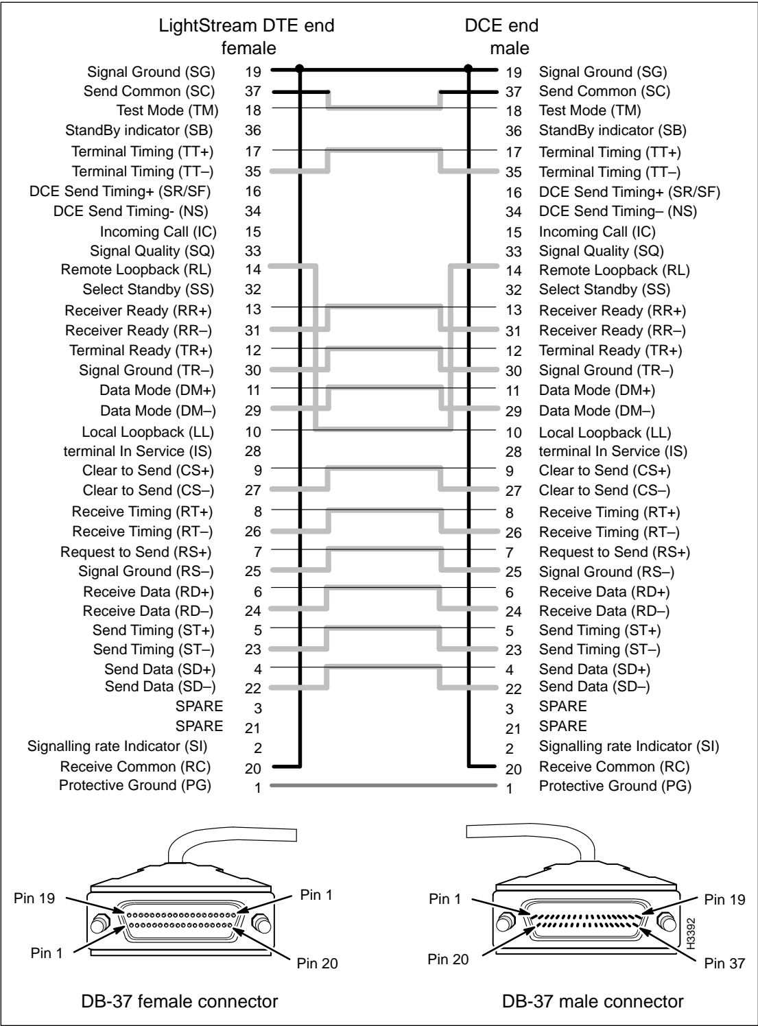
Figure 3-11 RS-449 Straight-through Cable Signal Diagram
