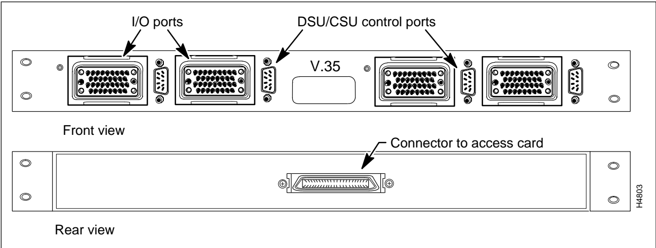
Figure 3-7 V.35 Fantail
