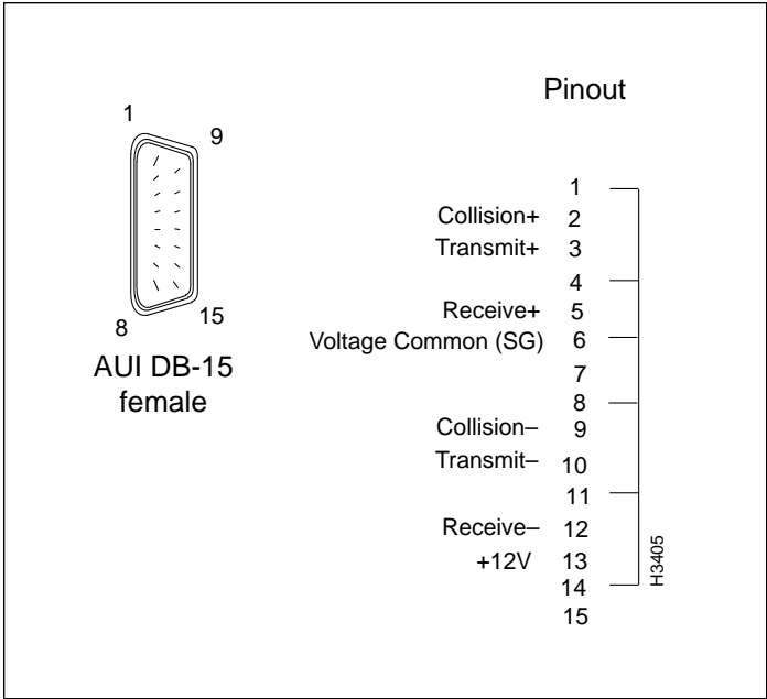
Figure 3-31 Ethernet Access Card AUI Connector Pin Assignments
