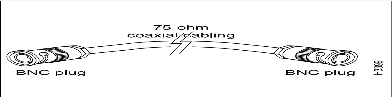
Figure 3-16 75-ohm Coaxial Data Cable
