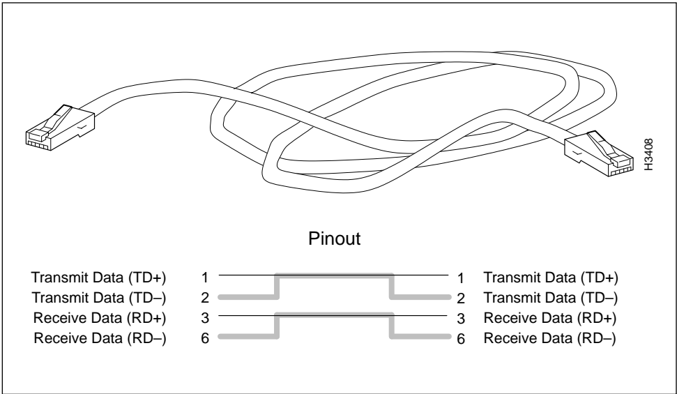
Figure 3-29 Ethernet 10BaseT Straight-through Cable and Pin Assignments
