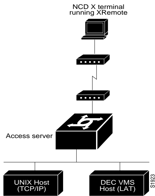
Figure 1-3 XRemote Connection
