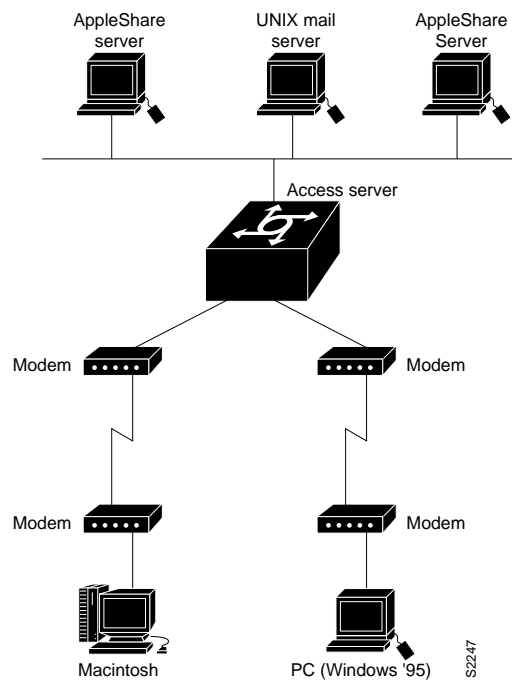
Figure 1-4 Telecommuting Connection
