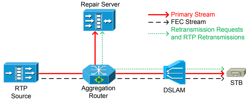
Fig. 1. A hybrid error-control method for IPTV systems running over DSL.
