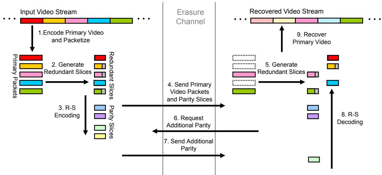
Fig. 3. Packet-level illustration of the proposed SLEP/SLEPr scheme.
