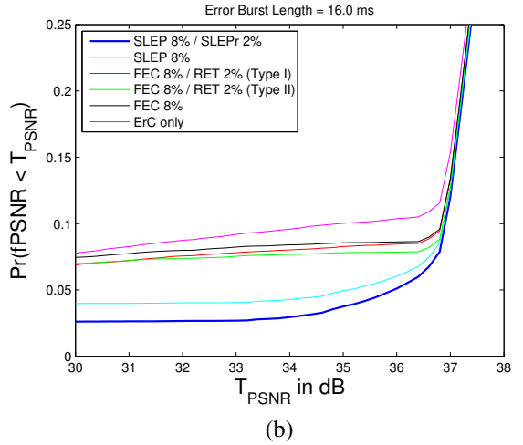
Fig. 7. CDF of fPSNR for SLEP/SLEPr and other schemes, (a) average burst length = 8 ms, (b) average burst length = 16 ms.
