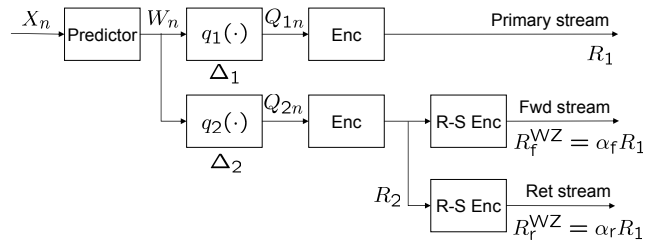
Fig. 4. Block diagram of the analytical model of the SLEP/SLEPr encoder.
